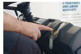
STEP 5 Sit on the seat to engage and turn key to ON position
